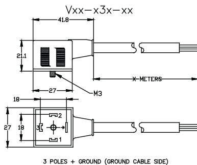
3 POLES + GROUND (GROUND CABLE SIDE)
