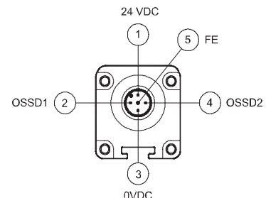
Receiver - 5 poles
