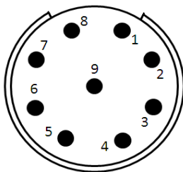
Male Pin Out (Front View)
