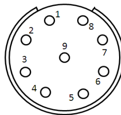
Female Pin Out (Front View)
