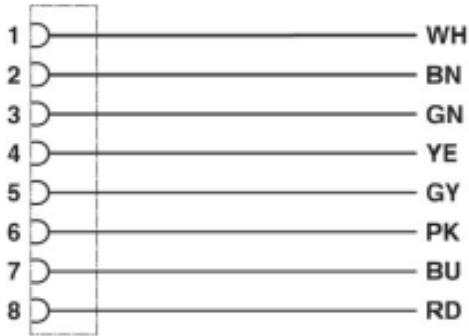
Pin Configuration
