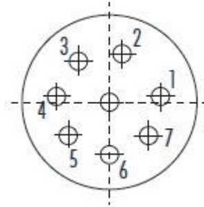
Connector Pinout (Front View)
